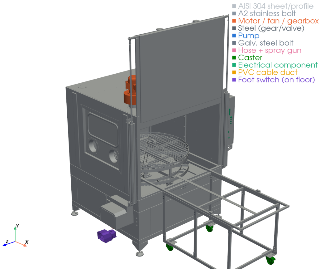
Figure 1. 3D view of the assembly coloured by material class (grey: AISI 304 sheet/profile).
