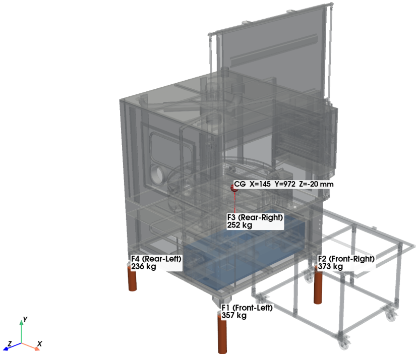
Figure 7. Case C (water + 300 kg basket load, 1,218 kg).
