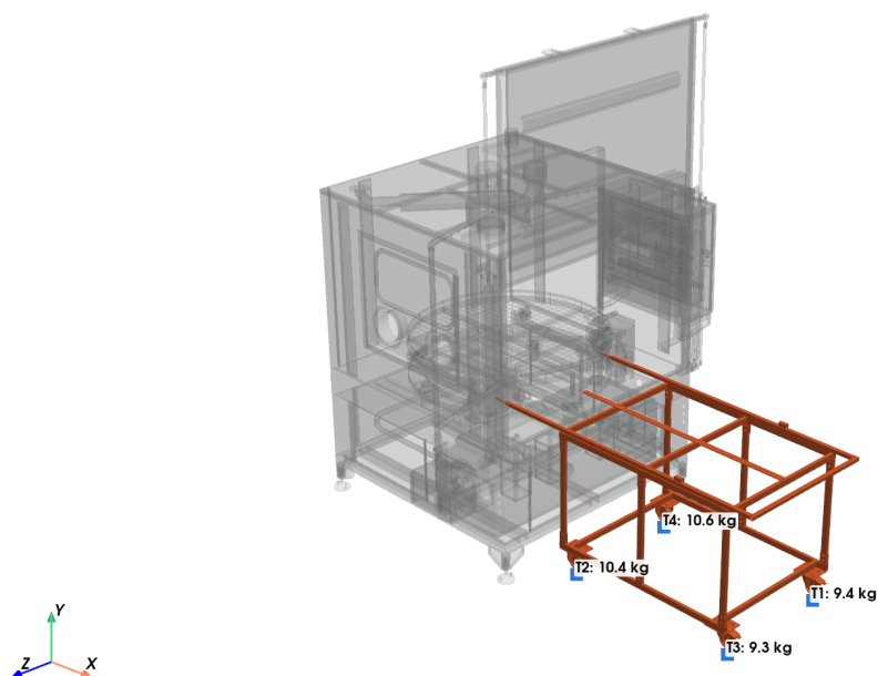
Figure 11. Loading trolley C011459 (39.7 kg) — its own caster loads T1-T4; no load on the machine feet.
