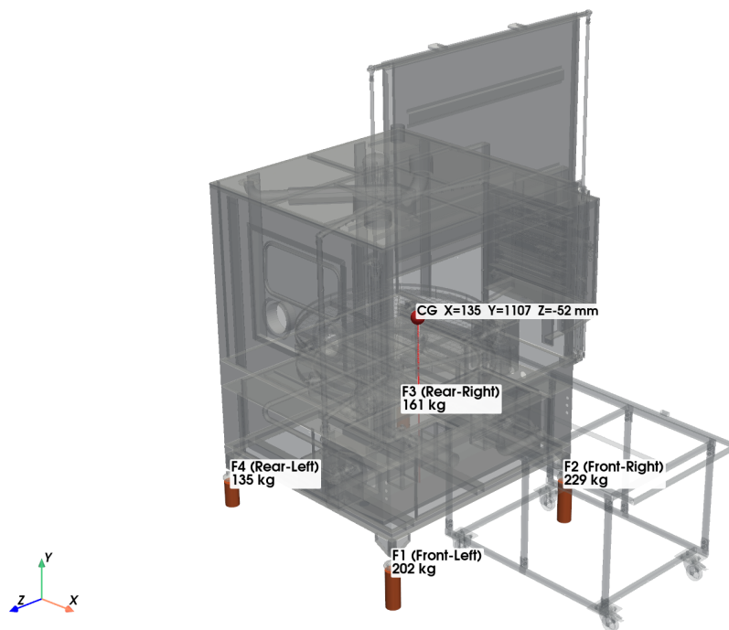
Figure 5. Case A (dry machine, 727 kg): CG position and foot loads; the height of the orange cylinders is proportional to the load.
