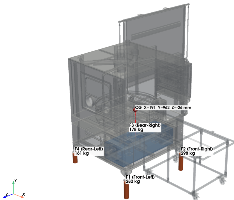
Figure 6. Case B (tank filled, 918 kg): the water volume is shown as a blue box.
